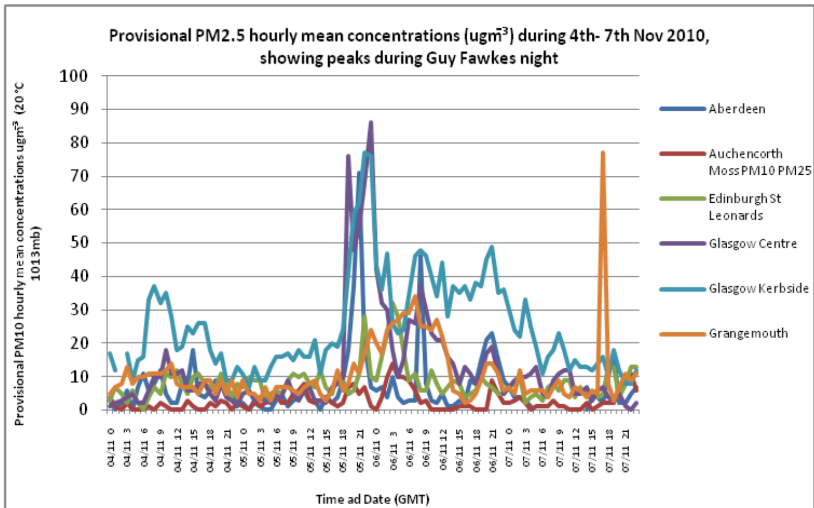
Figure 3: A graph showing the provisional PM2.5 concentrations observed throughout Scottish air quality monitoring sites on Guy Fawkes Night 2010
