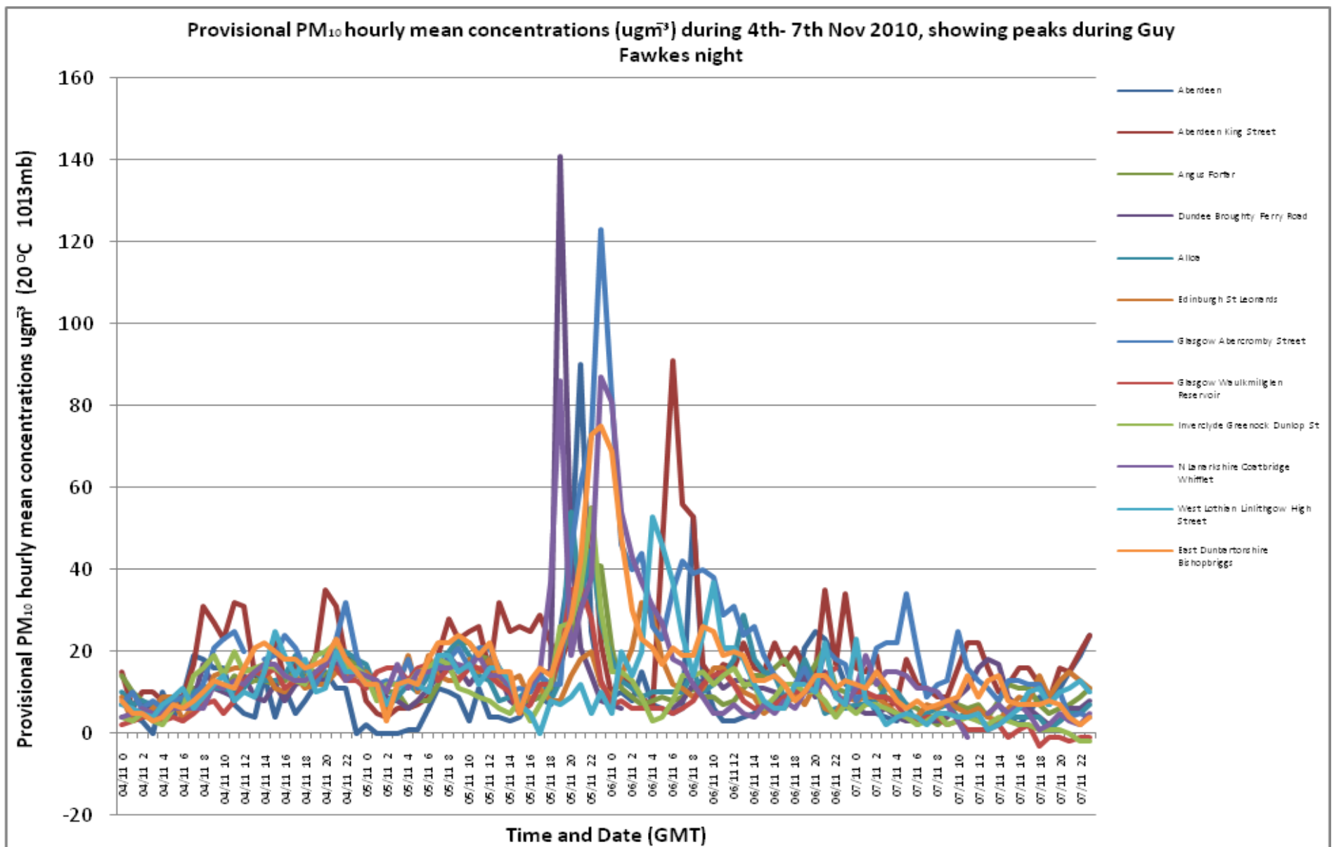
Figure 2: A graph showing the provisional PM 10 concentrations observed throughout a range of Scottish air quality monitoring sites on Guy Fawkes Night 2010
